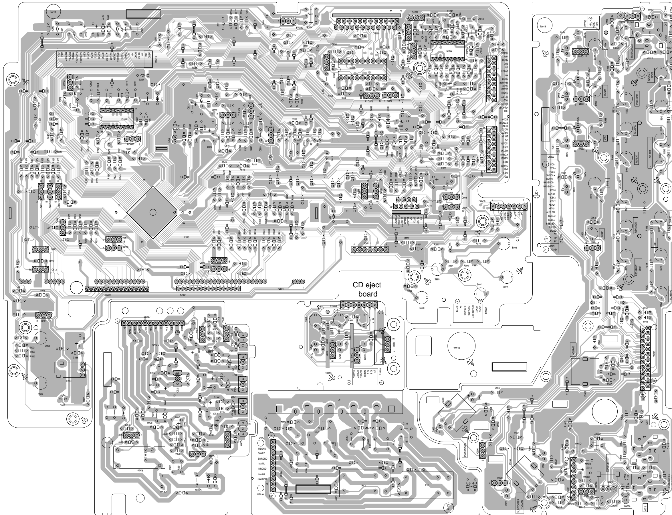
Voltage board
